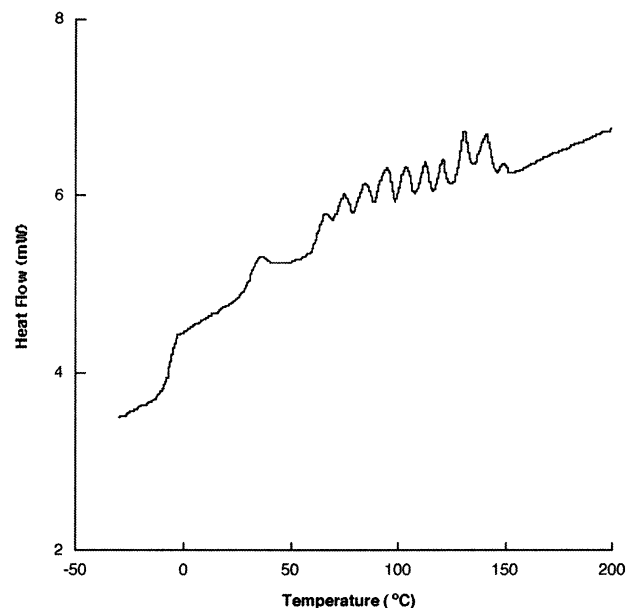
FIGURE 8. Thermal fractionation DSC of PP10-HS.
