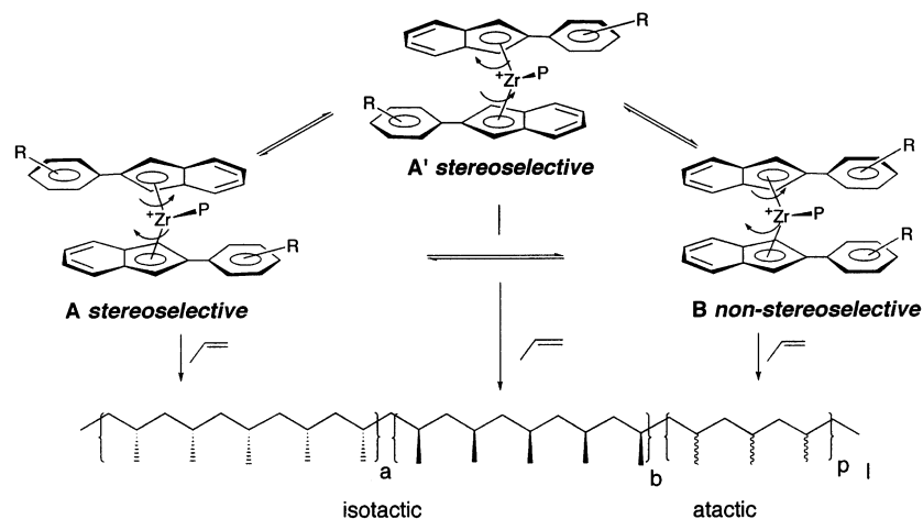
Scheme 2. Proposed Mechanism for Propylene Enchainment by (2-Arylindenyl) 2 ZrCl 2 Metallocenes
